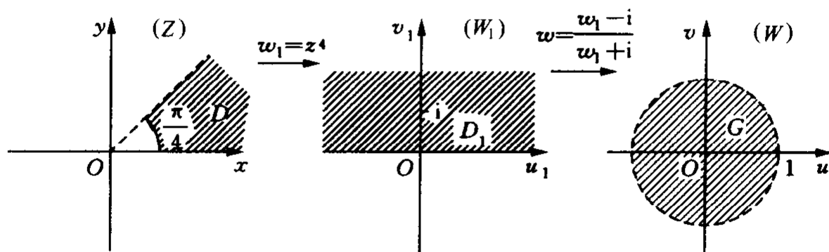
图 6-39 w = \frac{z^4 - i}{z^4 + i}
