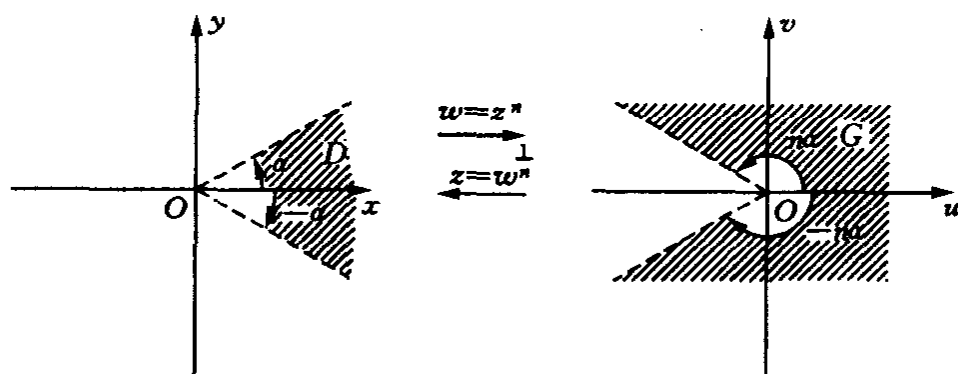
图 6-13 映射 w = z^n 与 z = w^{\frac{1}{n}} , 当 0 < \alpha < \frac{\pi}{n} 时,
