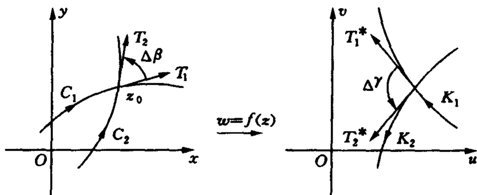
图 6-3 w = f(z) 在 z_0 点解析, f'(z_0) = \cdots = f^{(k-1)}(z_0) = 0 , f^{(k)}(z_0) \neq 0 , \Delta\gamma = k\Delta\beta
