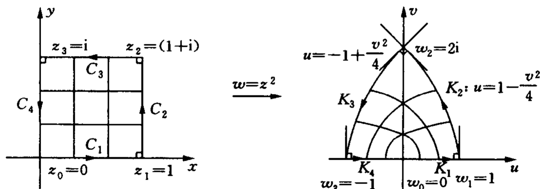
图 6-15 w = z^2
