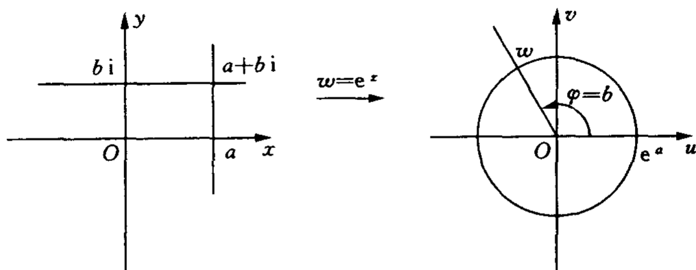
图 6-16 映射 w = e^z
