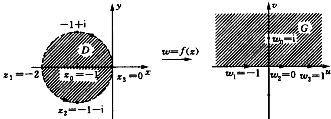
图 6-17 w = f(z) = \frac{(1-i)z+2}{(1+i)z+2}
