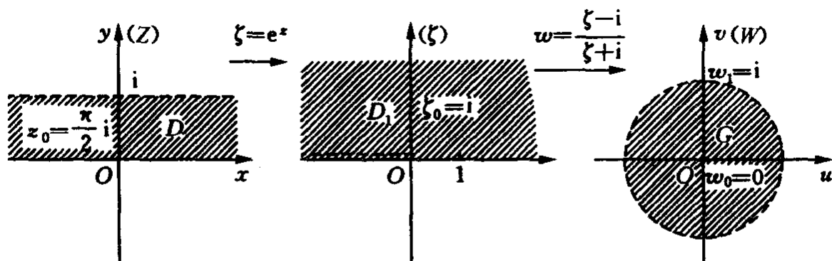
图 6-19 映射 w = \frac{e^z - i}{e^z + i}
