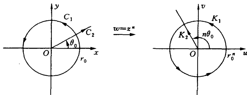
图 6-12 映射 w = z^n
