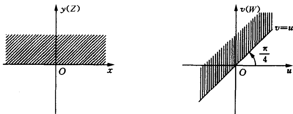
图 6-31 w = (1+i)z
