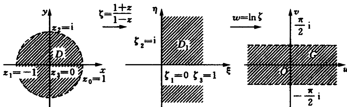
图 6-20 映射 w = \ln\left(\frac{1+z}{1-z}\right)
